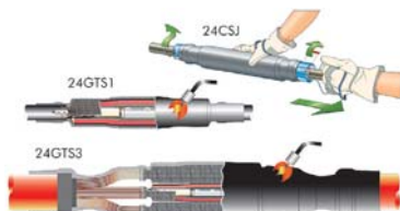
Joints from 10 kV to 42 kV and 25 mm 2 to 1200 mm 2
