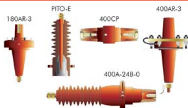
Equipment bushings from 10 kV to 42 kV
